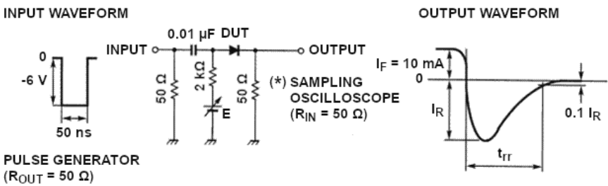
Fig. 5.1 Reverse recovery time ( t_{rr} ) Test circuit
