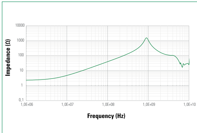
Impedance Curves
