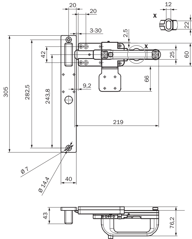
Dimensional drawing (Dimensions in mm (inch))
