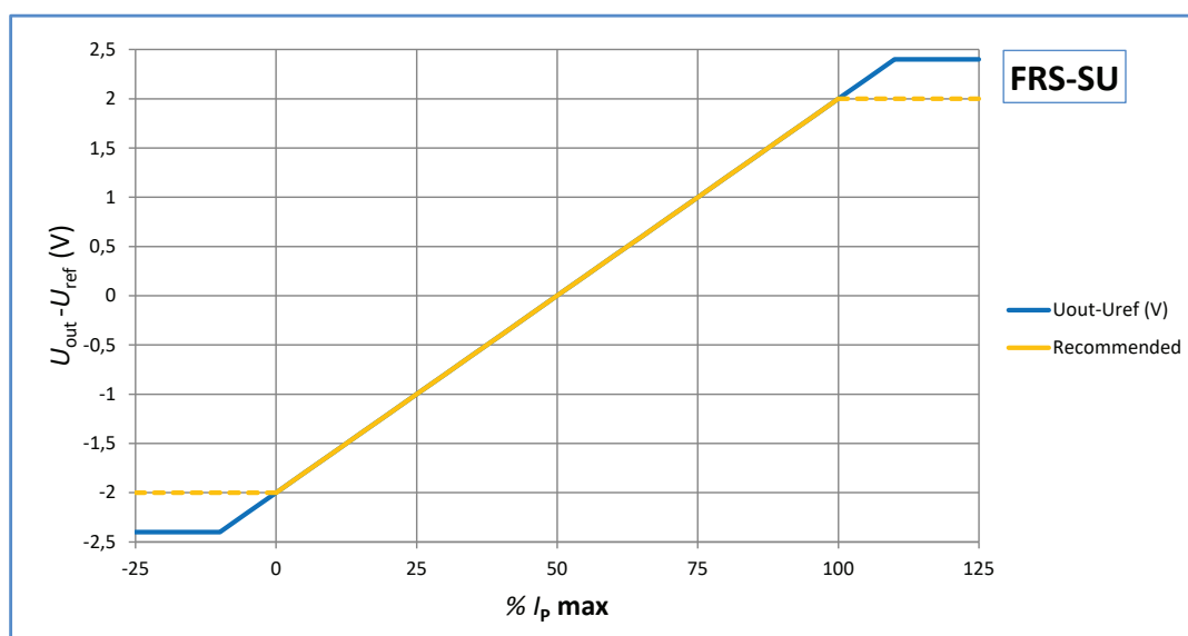
Figure 2: Uni-polar output current ( U_{out} - U_{ref} ) VS primary current I_p
