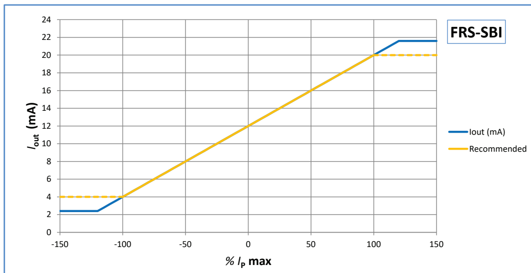
Figure 1: Bi-polar output current I_{out} VS primary current I_p
