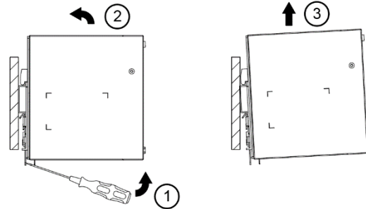
Fig. 3.2 Dismounting
