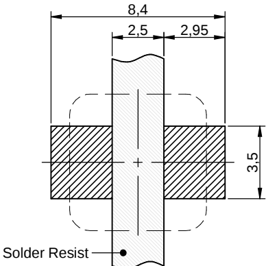
No vias and traces in restricted area Scale- 2:1
