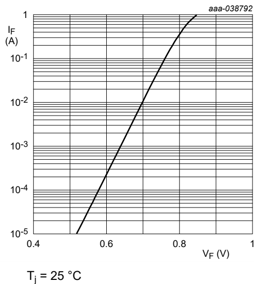
Fig. 3. Forward current as a function of forward voltage; typical values (HPZR-C3V3-Q)
