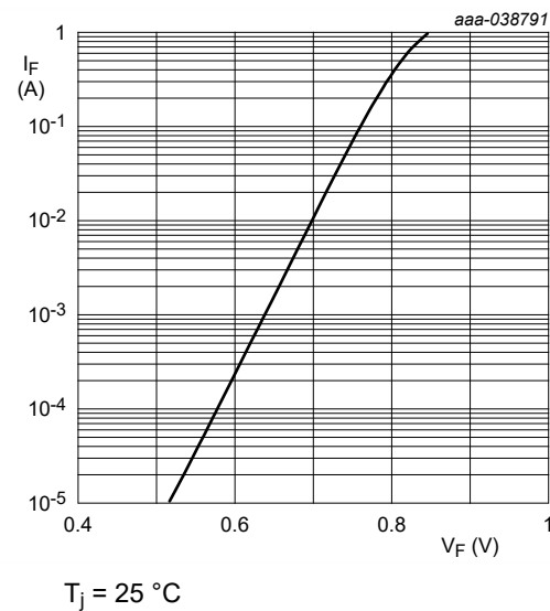
Fig. 2. Forward current as a function of forward voltage; typical values (HPZR-C3V0-Q)
