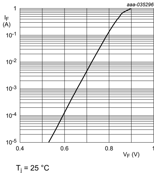
Fig. 8. Forward current as a function of forward voltage; typical values (HPZR-C68-Q)
