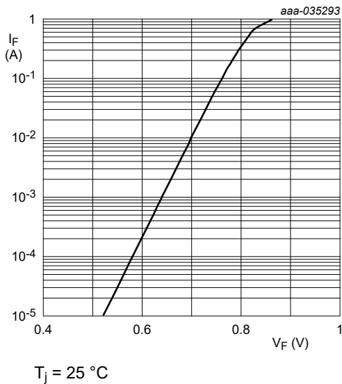
Fig. 5. Forward current as a function of forward voltage; typical values (HPZR-C5V6-Q)
