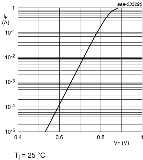
Fig. 7. Forward current as a function of forward voltage; typical values (HPZR-C8V2-Q)
