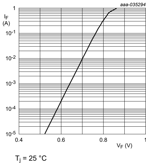
Fig. 6. Forward current as a function of forward voltage; typical values (HPZR-C7V0-Q)
