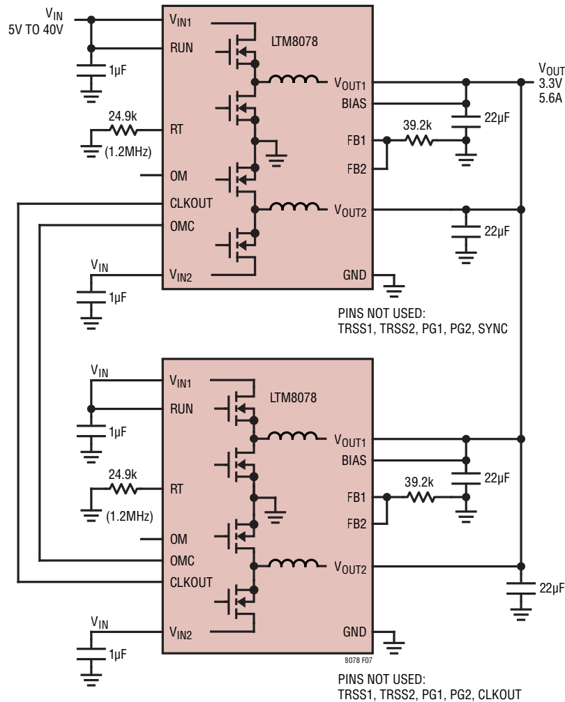
Figure 7. Parallel All Channels of Two LTM8078 to Produce 3.3V, 5.6A from 5V to 40V Input, BIAS Connected to V_{OUT}
