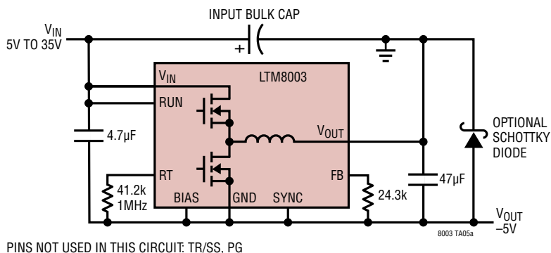
-5V OUT from 5V IN to 35V IN Positive to Negative Converter, BIAS tied to LTM8003 GND
