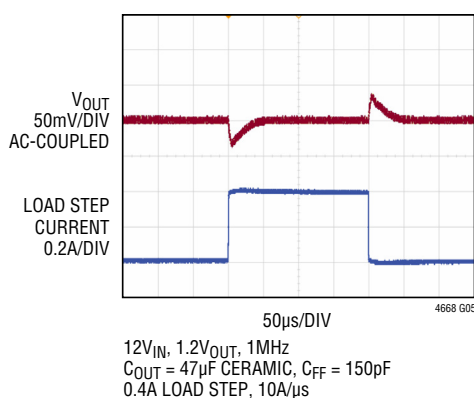
1.2V Output Transient Response
