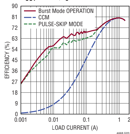
Burst Mode Operation and Pulse Skip Mode Efficiency, V IN = 12V, V OUT = 1.5V, f S = 1MHz
