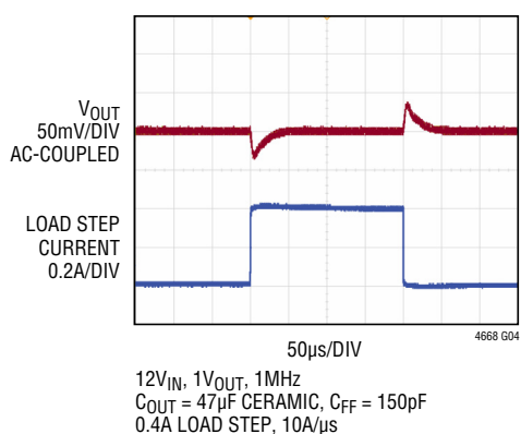
1V Output Transient Response
