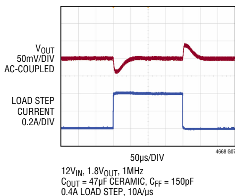
1.8V Output Transient Response
