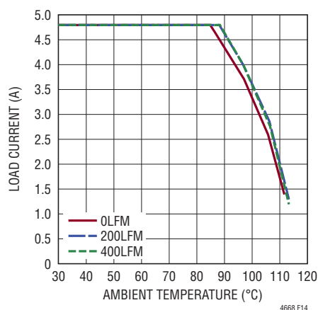
Figure 14. 12V to 1.2V Derating Curve, No Heat Sinking
