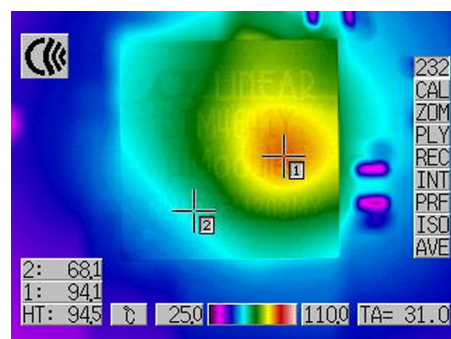
Figure 55. Thermal Image of U1 from Figure 51 Circuit. Delivering 6V OUT at 10A from 36V IN , with 6V OUT Feeding INTV CC /DRV CC Through D1c Diode. T A = 25°C, Bench Testing, No Airflow
