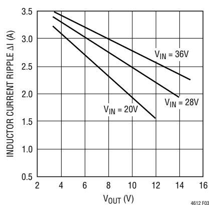
Figure 3. Inductor Current Ripple vs Output Voltage
