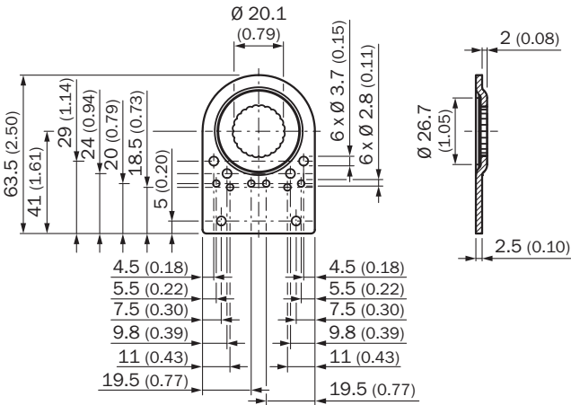
Dimensional drawing (Dimensions in mm (inch))
