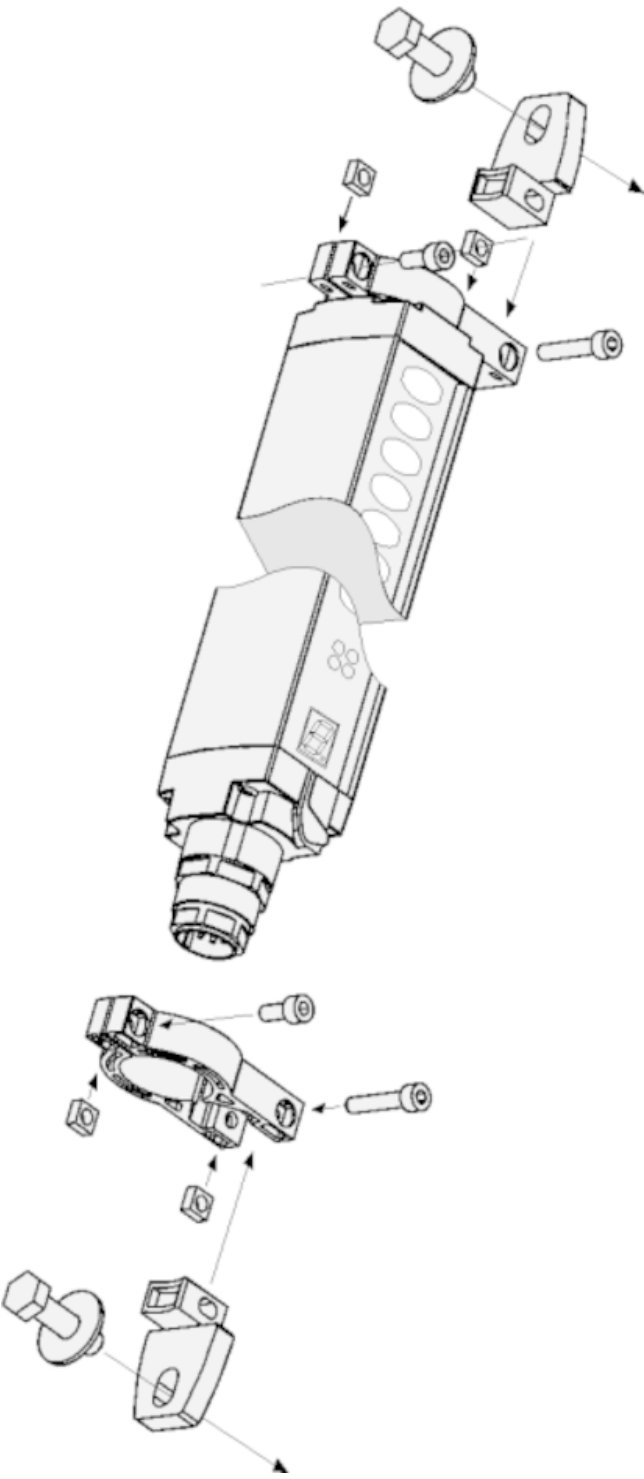
Exploded view
