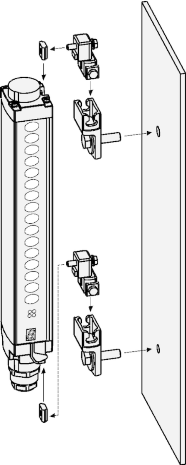
Exploded view
