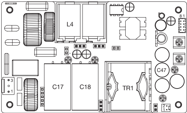
Upper PCB
