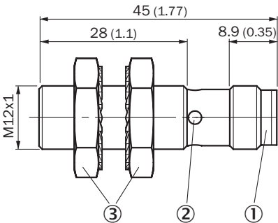
IMB12 Short-body housing, connector M12, flush
