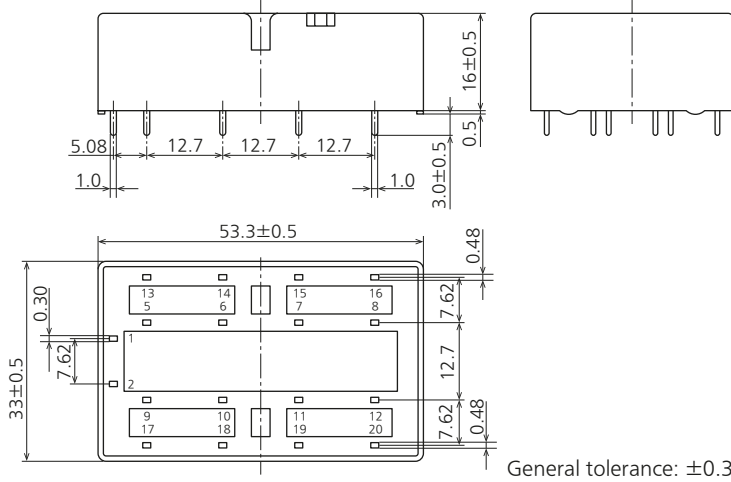
External dimensions
