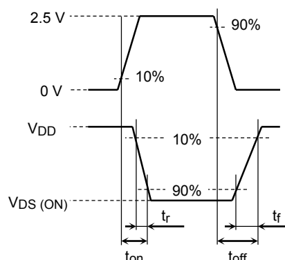
(c) V_{OUT}
