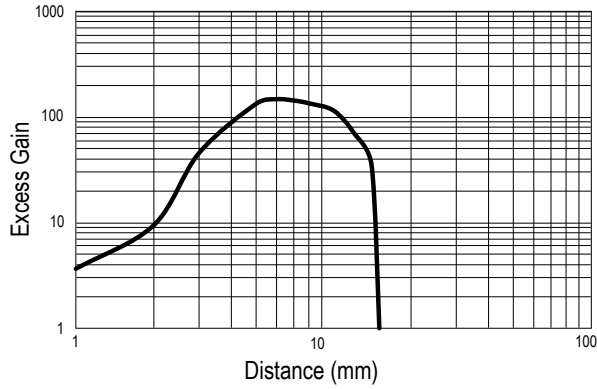
Excess Gain (15 mm Q2XABFF15-xx Models)
