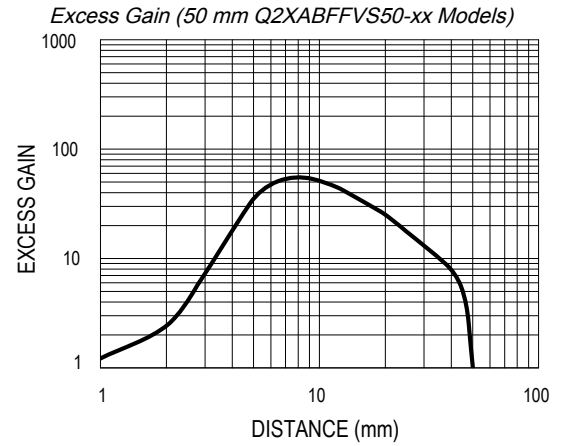
Typical Performance Spot size: 1.7 mm at 30 mm Cutoff variation due to 90%/6% color shift \leq 2.5 mm
