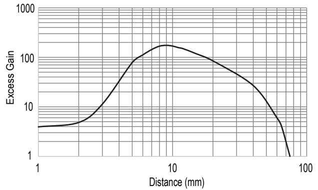
Excess Gain (75 mm Q2XABFF75-xx Models)
