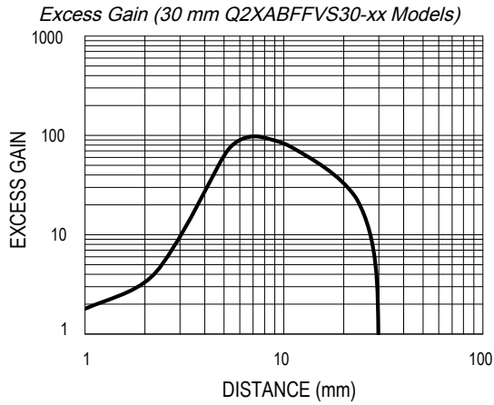
Typical Performance Spot Size: 0.9 mm at 15 mm Cutoff variation due to 90%/6% color shift \leq 0.75 mm
