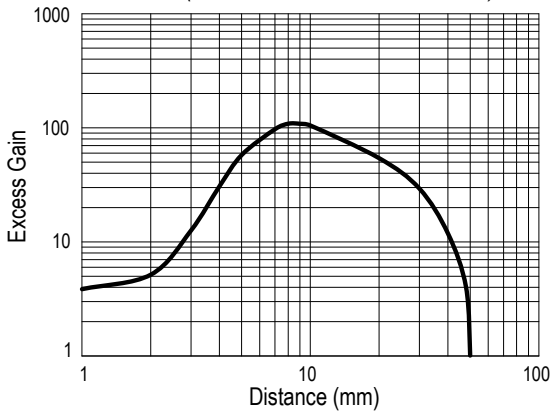
Excess Gain (50 mm Q2XABFF50-xx Models)
