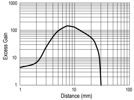
Excess Gain (30 mm Q2XABFF30-xx Models)
