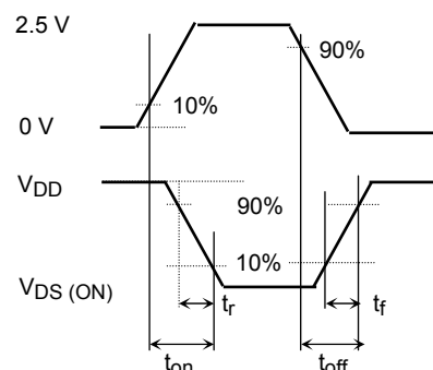
(c) V_{OUT}
