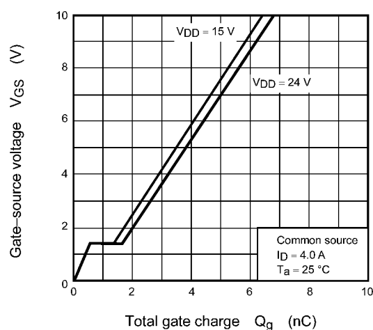
Fig. 8.1.11 Dynamic Input Characteristics
