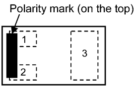
Fig. 6.1 Marking
