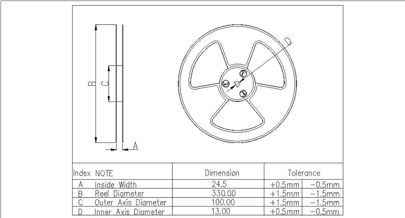
Figure 16 Reel dimensions
