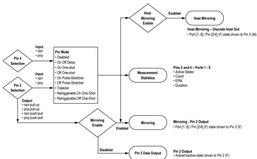
Figure 1. Logic Flow
