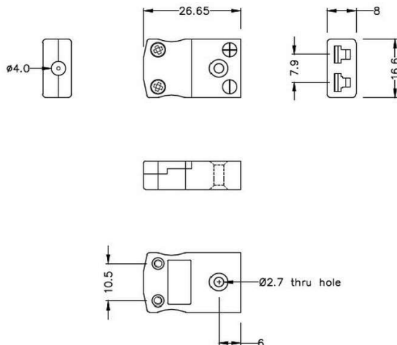
Miniature in-line Socket (dimensions in mm)
