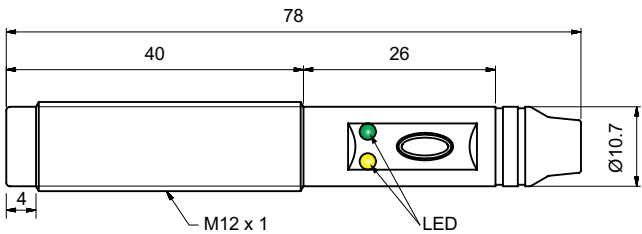
Fig. 7 Cable CA12EAN...A2IO
