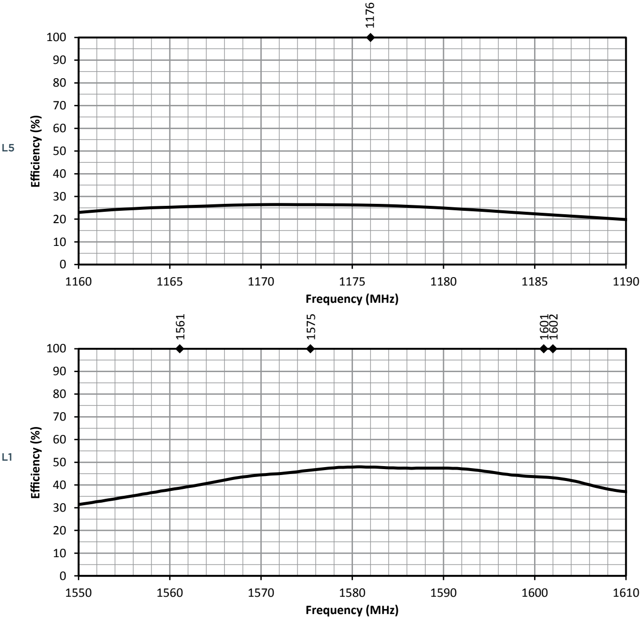
Figure 5. ANT-GNFPC-SHL15 Antenna Radiation Efficiency with Frequency Band Highlights
