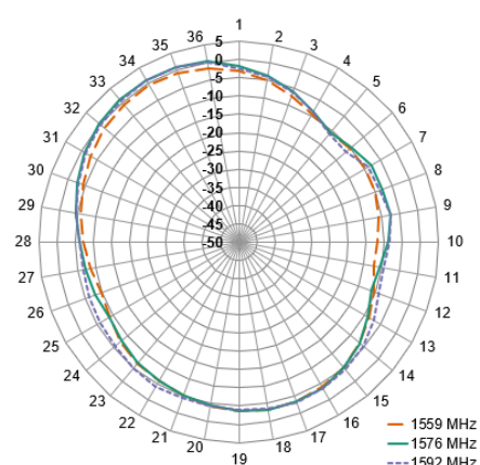
XY-Plane Gain
