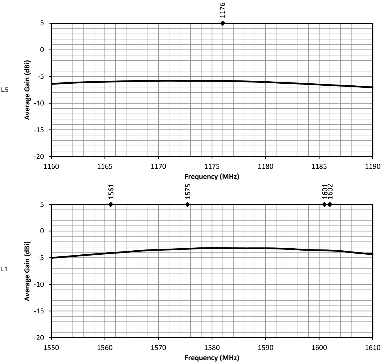
Figure 4. ANT-GNFPC-SHL15 Antenna Average Gain with Frequency Band Highlights
