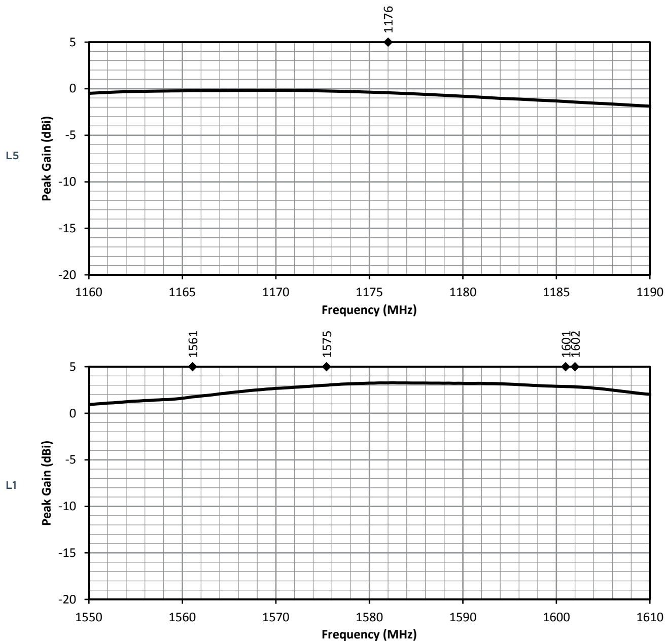
Figure 3. ANT-GNFPC-SHL15 Antenna Peak Gain with Frequency Band Highlights
