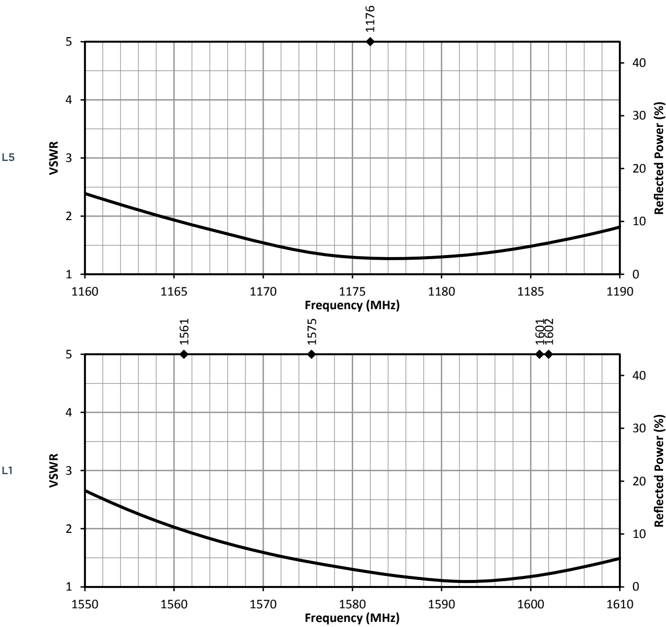
Figure 2. ANT-GNFPC-SHL15 Antenna VSWR with Frequency Band Highlights
