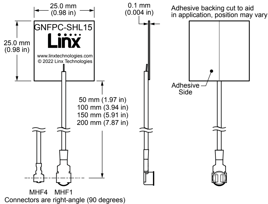
Figure 1. ANT-GNFPC-SHL15 Product Dimensions
