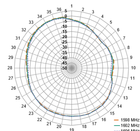
XY-Plane Gain
