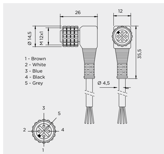
M12 female 90° angle connector 5-pole
