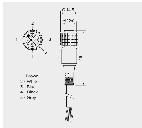
M12 female straight connector 5-pole
