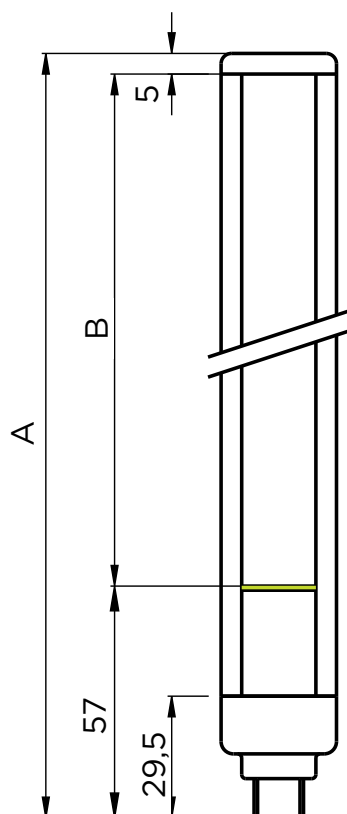
Emitter - Receiver
