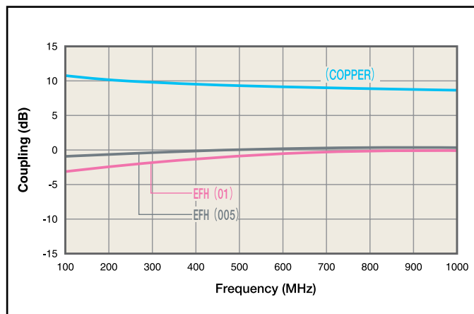
EFH – Attenuation of coupling noise
