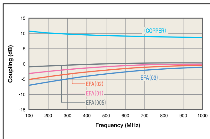
EFA – Attenuation of coupling noise
