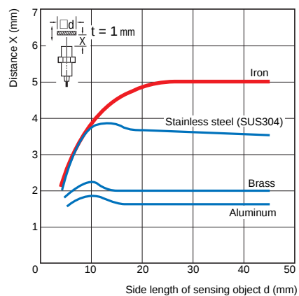
E2E2-X5MC□/I-X5MY□
