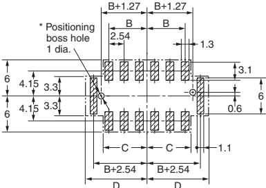
PCB Mating Dimensions (TOP VIEW)
