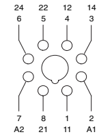
Terminal Arrangement
