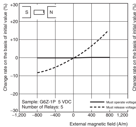
External Magnetic Interference (Average value)
