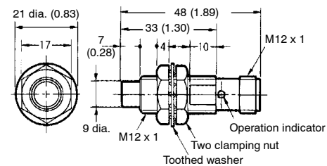
Fig.17: E2E-X10ME□-M1/F□-M1
