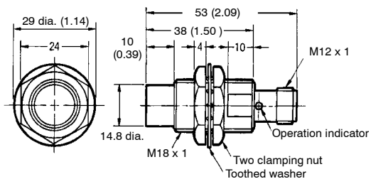
Fig.17: E2E-X10ME□-M1/F□-M1
