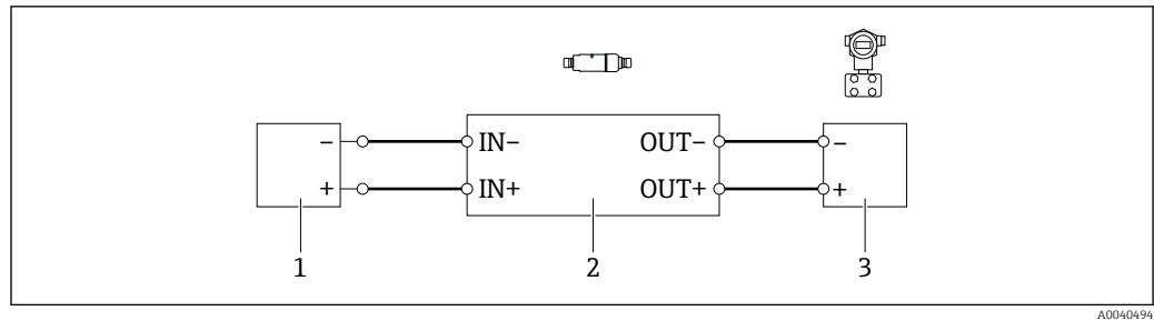
4 Electrical connection for 2-wire HART field devices with passive current output (optional grounding not shown)
