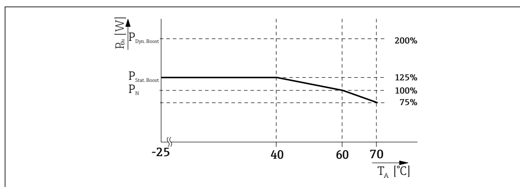
5 Output power depending on the ambient temperature
