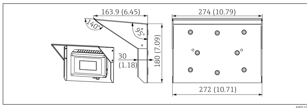
5 Dimensions in mm (in)
