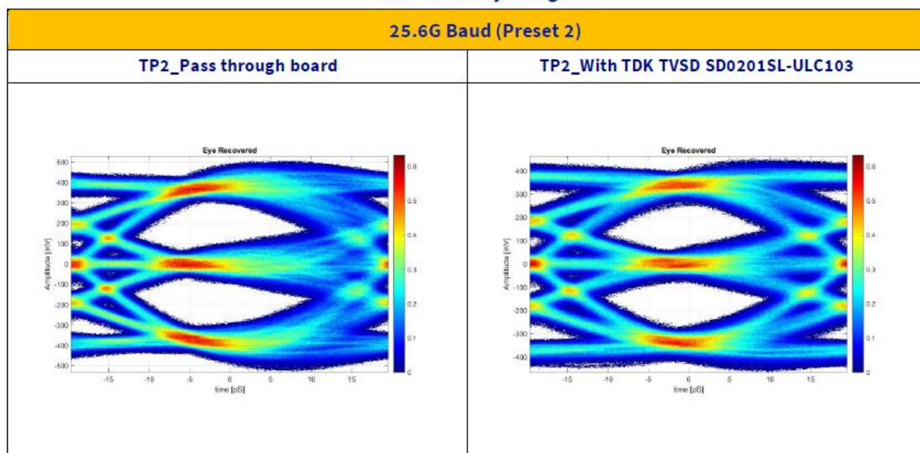
25.6G Baud Eye Diagram
