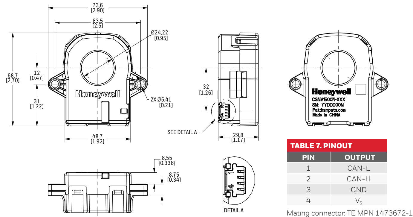
Figure 3. Dimensional Drawings (For reference only: mm)
