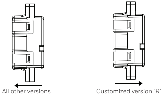
Figure 5. I_p Positive Primary Current Direction (Polarity)
