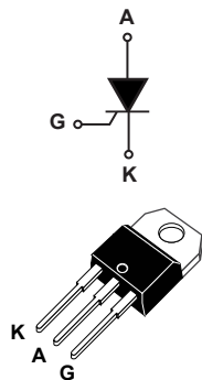
TO-220AB insulated
