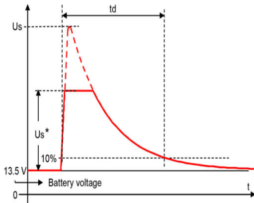
Figure 17. ISO7637-2 pulse 5b definition
