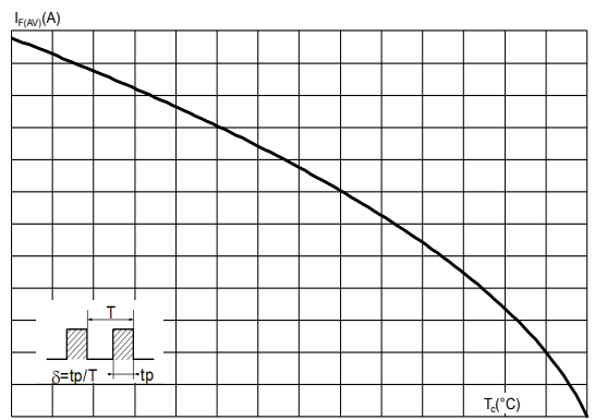
Figure 4. Average forward current versus case temperature ( \delta = 0.5 , PSMC)
