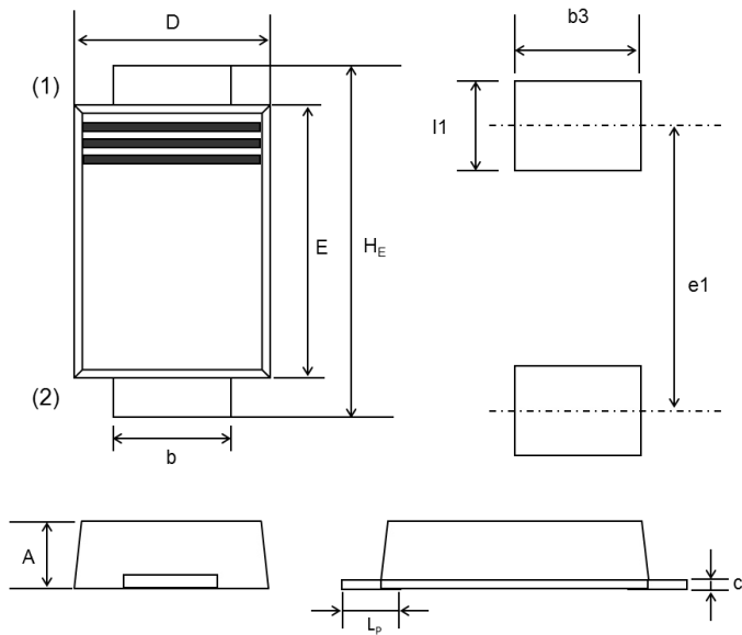
SOD-128, (PMD™)
