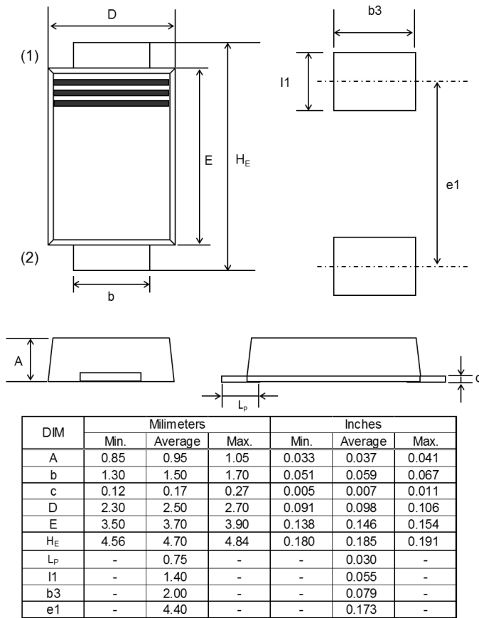
SOD-128, □, (FVDTM)
