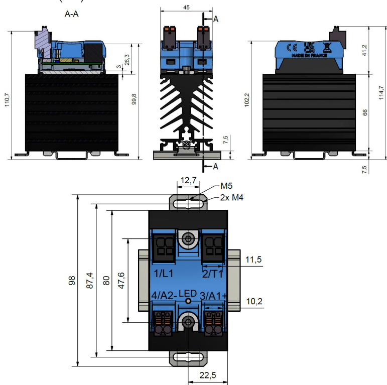
Dimensions (mm)
