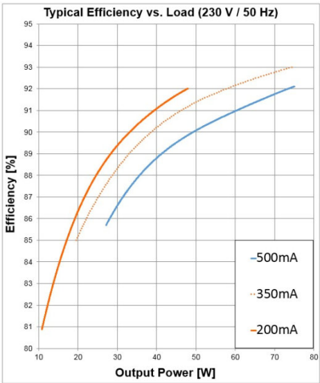
Typical Efficiency vs. Load (230V50Hz) OTI DALI 75220-240500 D NFC FL
