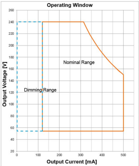
Operating Window OTI DALI 75220-240500 D NFC FL
