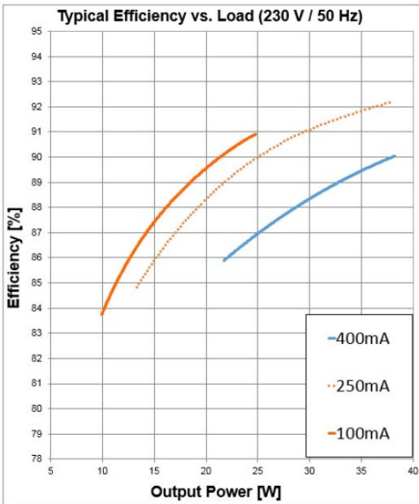
Typical Efficiency vs.Load (230V50Hz) OTI DALI 35220-240400 D NFC FL
